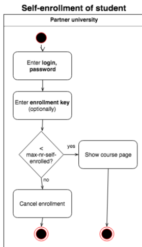
Figure 8: Workflow - Self Enrollment
