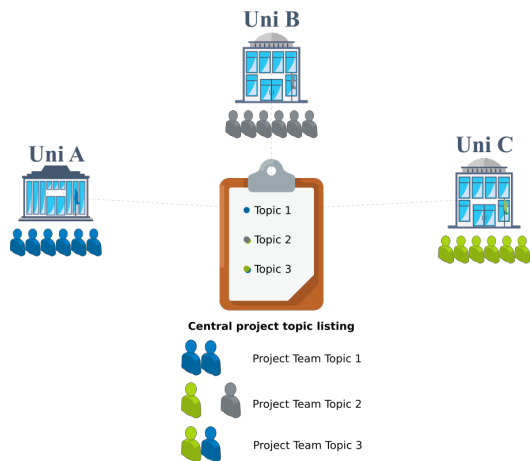
Figure 12: Workflow - Overview
