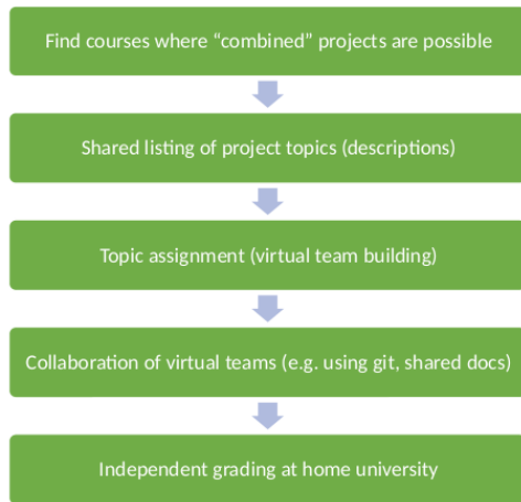
Figure 10: Workflow - Main
